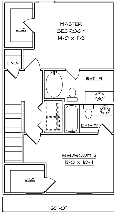
2nd FLOOR
